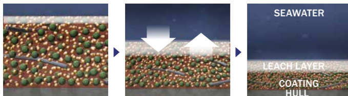
Seawater penetrates the coating and activates the binder (yellow) and biocide (green). The binder dissolves and the biocide leaches out of the coating and polishes stably.
