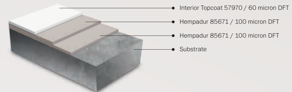
System 3 - Bilges
